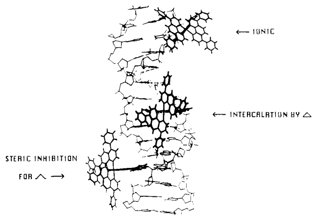
Figure 9. Enantiomeric selectivity for \text{Ru}(\text{DIP})_3^{2+} in binding to B-DNA. Top: Ionic binding of \Lambda isomer to the sugar-phosphate backbone. Middle: Intercalation of \Delta isomer into the double helix. Bottom: Steric inhibition of intercalation of \Lambda isomer into the helix.
